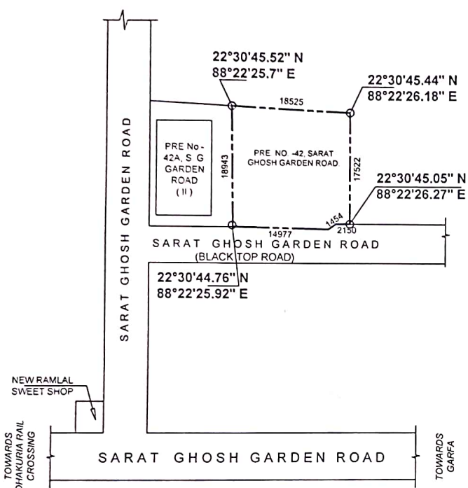
SITE PLAN. (SCALE = 1: 600)
